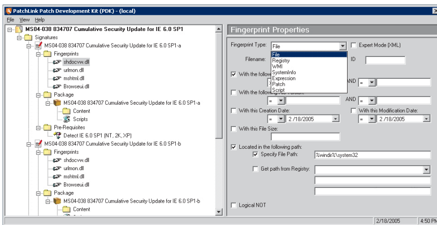
PatchLink Developers Kit
